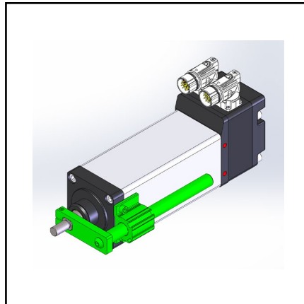
Anti-Rotate Kit
